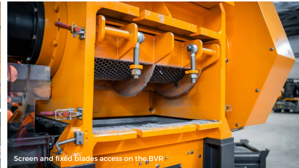
Screen and fixed blades access on the BVR
